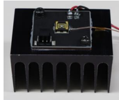
Picture 5. Fins facing down (This orientation obstructs the air flow)
