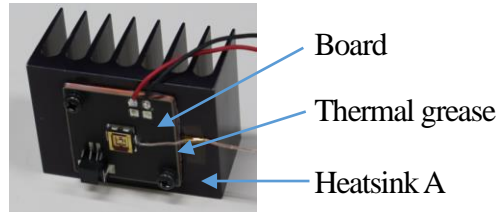
Picture 2. Evaluated light source 4-1
