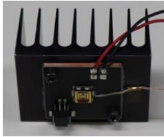
Picture 4. Fins facing vertical (Nichia uses this orientation)
